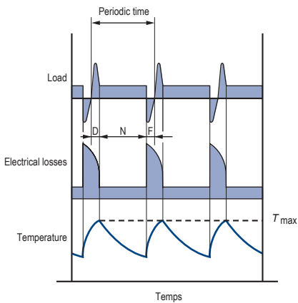
Fig. 7. - Periodic continuous duty with electrical braking. Type S7.
